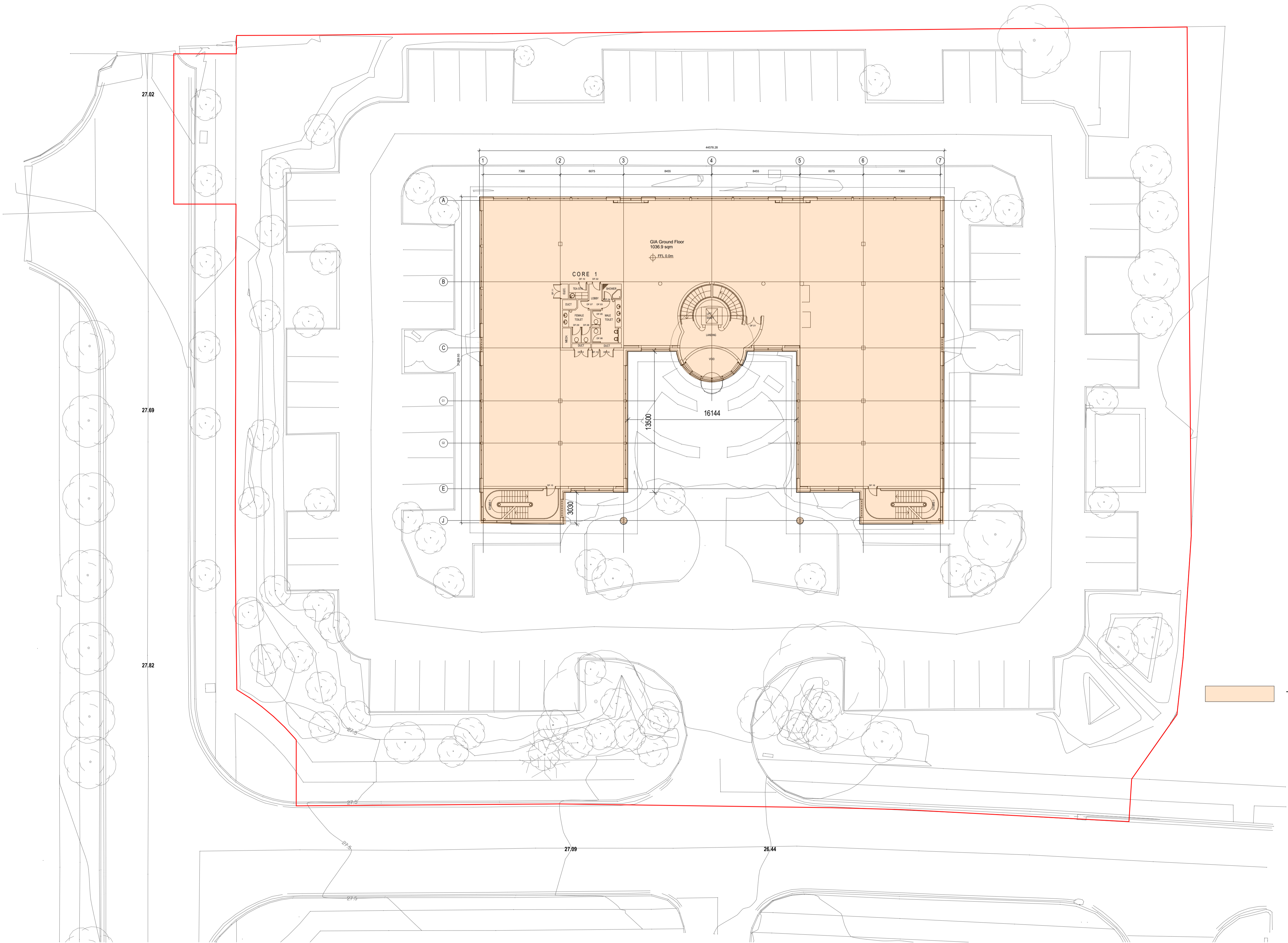
1 Demolition Ground Floor Plan 1 : 200
