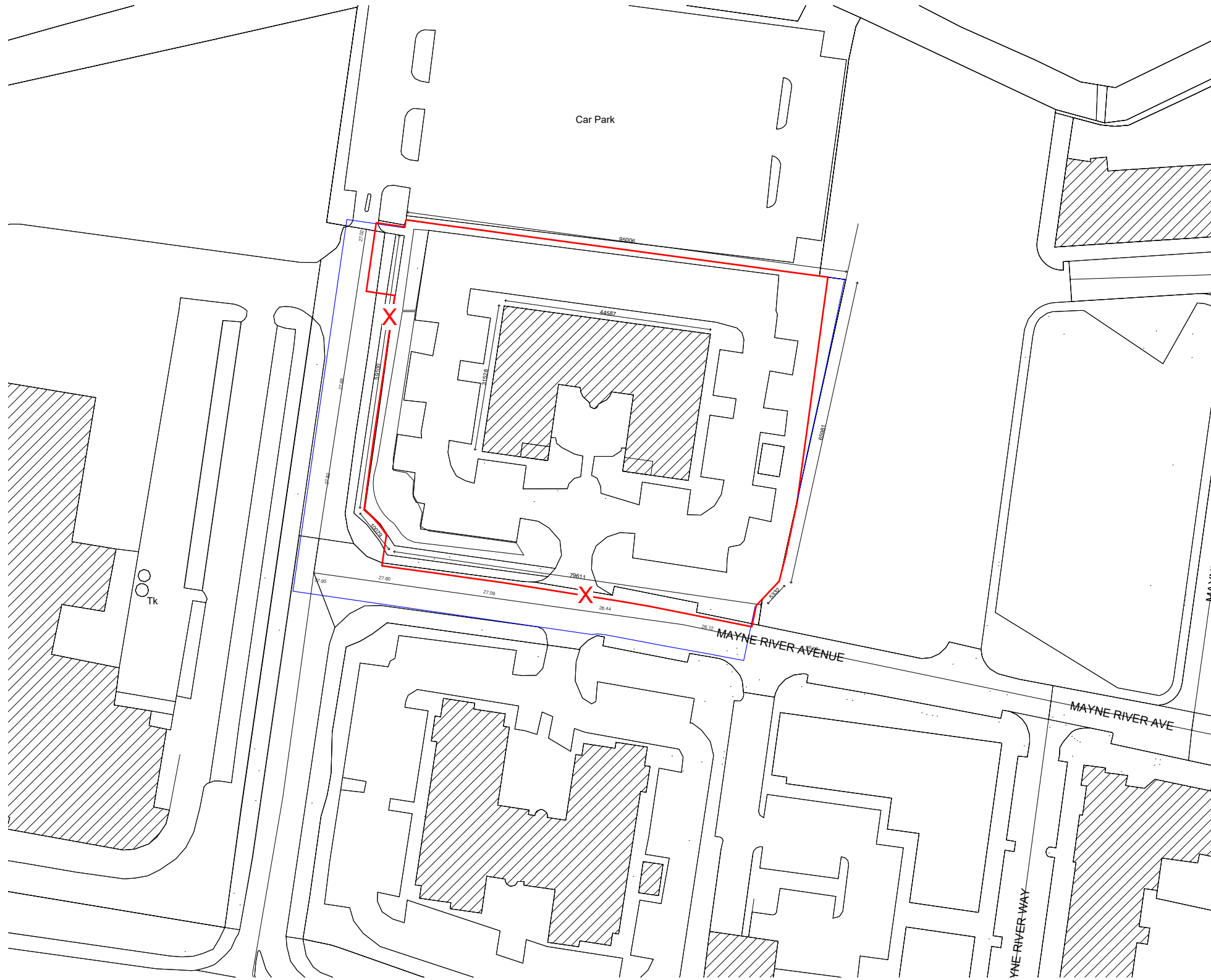
1 OS Site Location Map 1 : 1000
