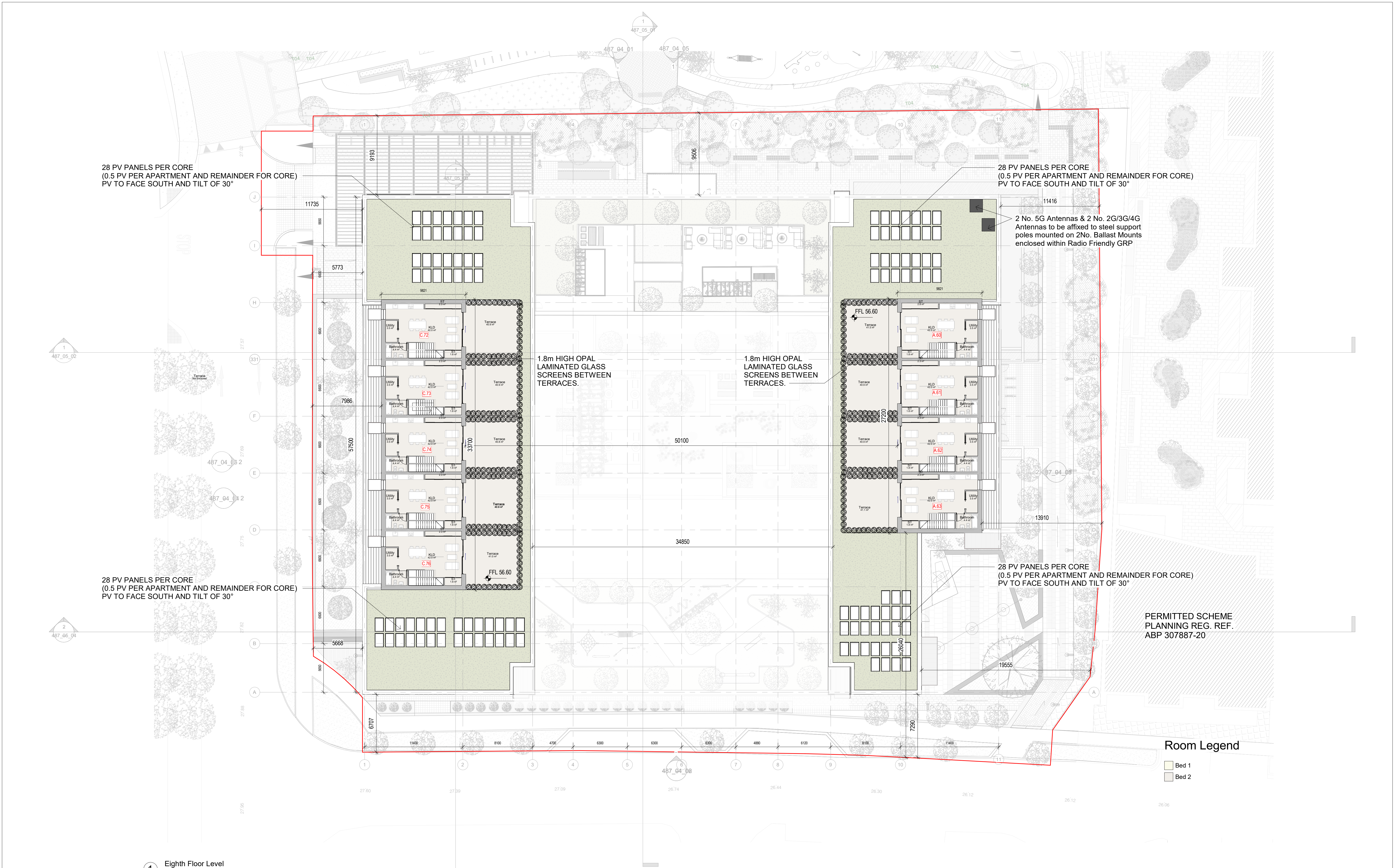
1 Eighth Floor Level 1 : 200
