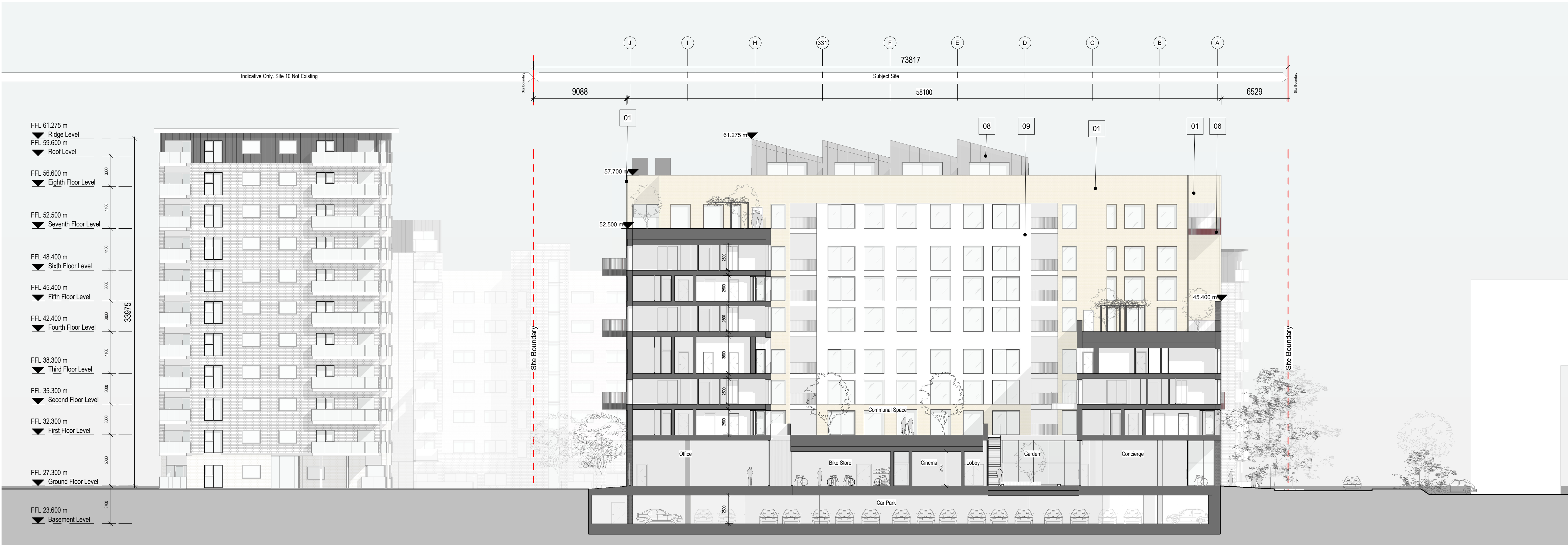
1 Section Facing East 1 : 200
